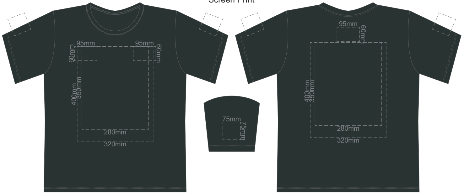
FRONT XL
